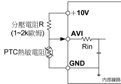
(b) PTC熱敏電阻連接
