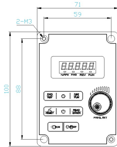
LED 数字操作器之外形尺寸图
