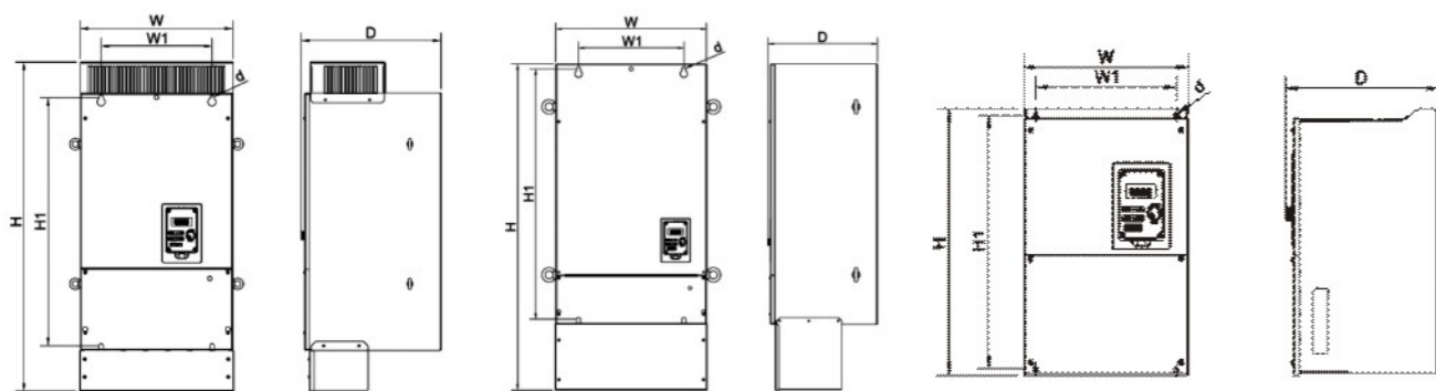
(图F)380V :100~125HP (IP20) (图G)380V :150~335HP (IP20) (图H)380V :375~535HP (IP20)
