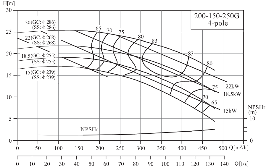
NIS/NISF200-150-250G/200-150-315G
