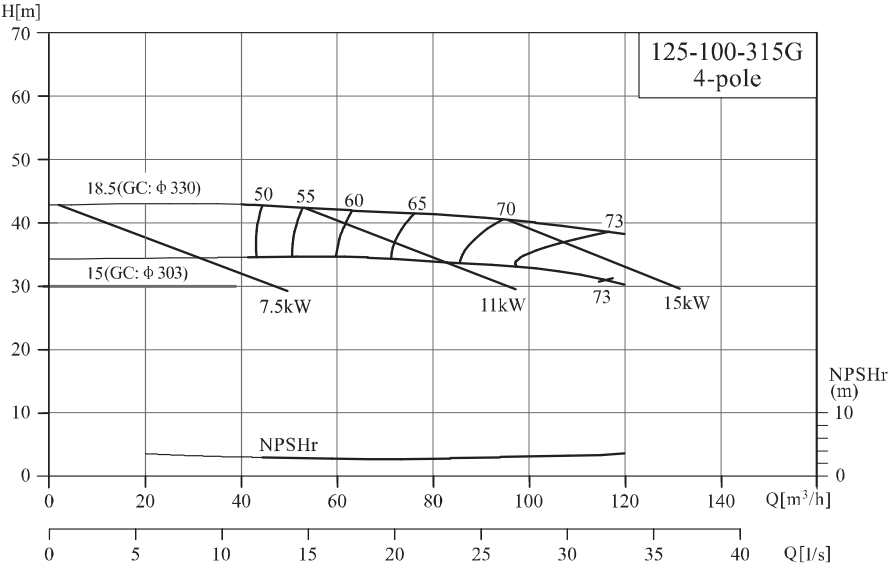
NIS/NISF125-100-315G/125-100-400G
