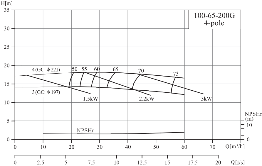
NIS/NISF100-65-200G/100-65-250G
