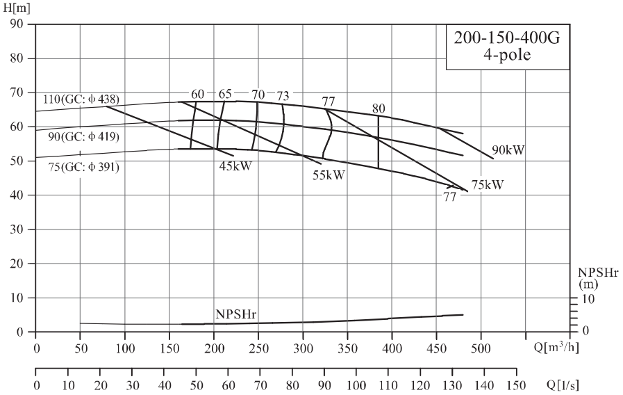
NIS/NISF200-150-400G
