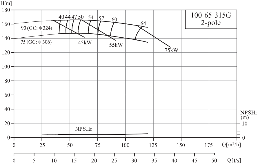
NIS/NISF100-65-315G/100-80-160G
