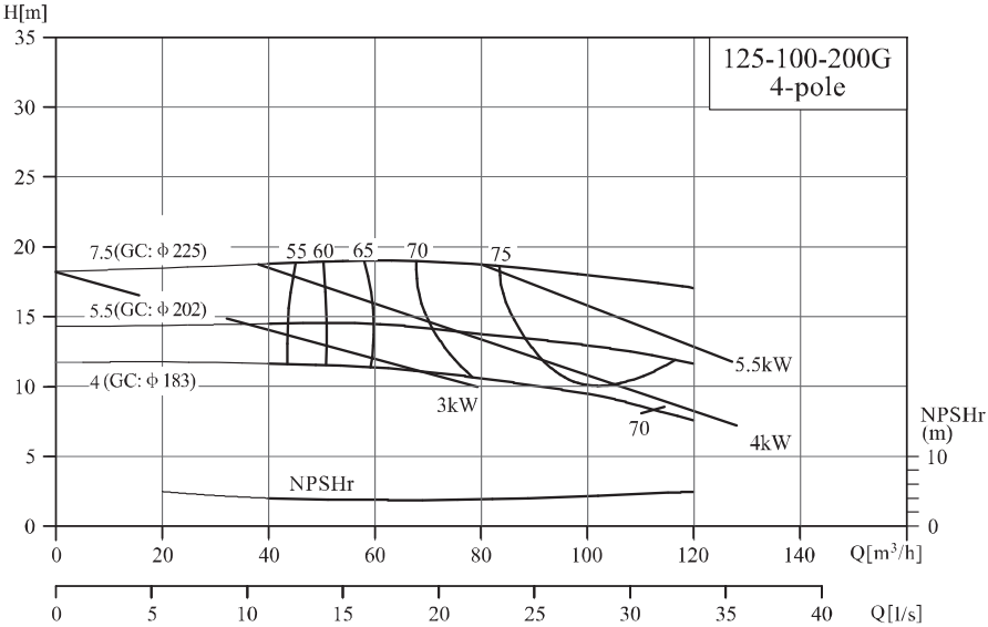
NIS/NISF125-100-200G/125-100-250G
