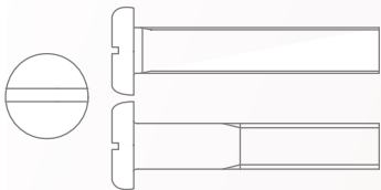
DIN85 SLOTTED PAN HEAD
